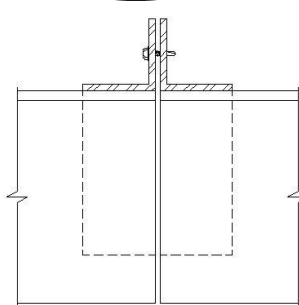
Invisible Mullion
