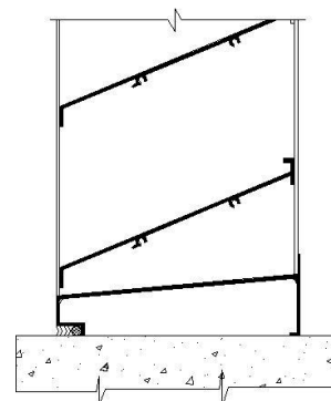
Channel Frame
