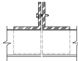
Invisible Mullion
