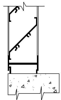
Channel Frame
