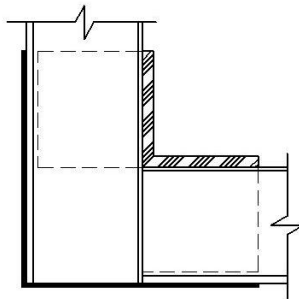
Post Corner
