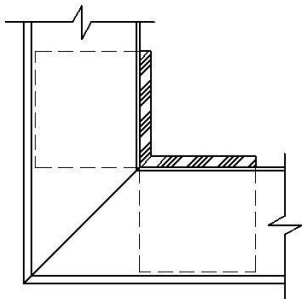
Mitered Corner
