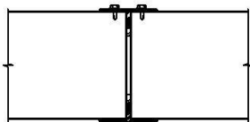
Exposed Mullion
